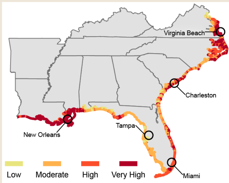
Figure 17.6. The map shows the relative risk that physical changes will occur as sea level rises. The Coastal Vulnerability Index used here is calculated based on tidal range, wave height, coastal slope, shoreline change, landform and processes, and historical rate of relative sea level rise. The approach combines a coastal system's susceptibility to change with its natural ability to adapt to changing environmental conditions, and yields a relative measure of the system's natural vulnerability to the effects of sea level rise. (Data from Hammar-Klose and Thieler 2001 18 ).
